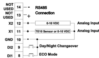
Wiring diagram for all applications Analog and Digital Inputs
