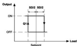
Application No. 1: Single RA On-Off Output
