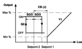
Application No. 9: RA On-Off Output & DA modulating Output
