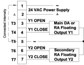
Wiring diagram for applications 6,7 and 8
