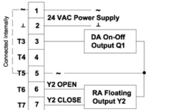
Wiring diagram for application 10
