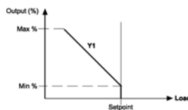
Application No. 6: Single RA Modulating Output
