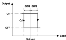
Application No. 1: Single RA On-Off Output
