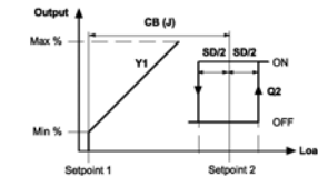
Application No. 12: DA Modulating Output & DA On-Off Output
