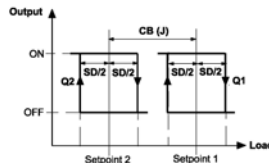
Application No. 3: Dual RA On-Off Outputs
