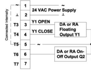
Wiring diagram for applications 9,11 and 12
