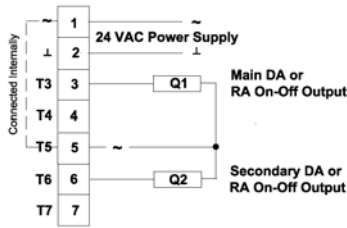
Wiring diagram for applications 1,2,3,4 and 5
