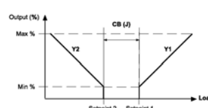
Application No. 8: RA Modulating & DA Modulating Output
