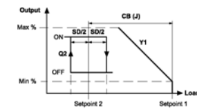
Application No. 11: RA On-Off Output & RA Modulating Output
