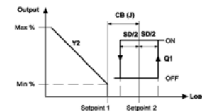
Application No. 10: RA Modulating Output & DA On-off Output
