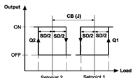
Application No. 5: RA On-Off & DA On-Off Output
