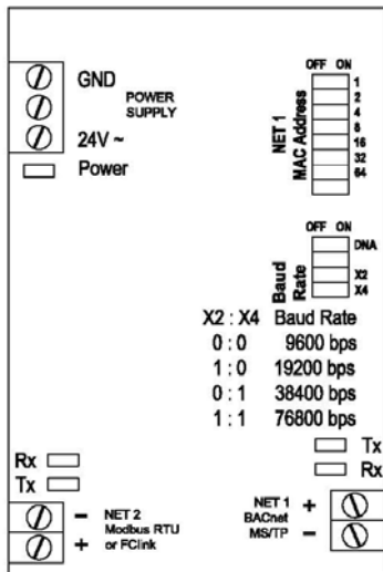
Termination Diagram
