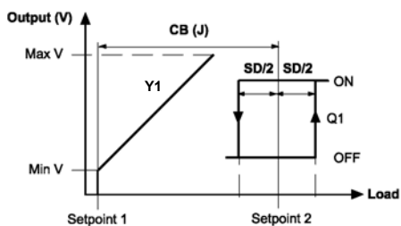
Application No. 9: DA On-Off + DA 0(2)-10 VDC Outputs
