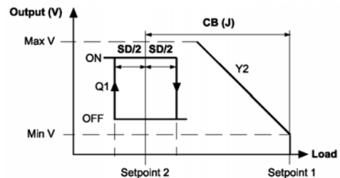
Application No. 8: RA On-Off + RA 0(2)-10 VDC Outputs
