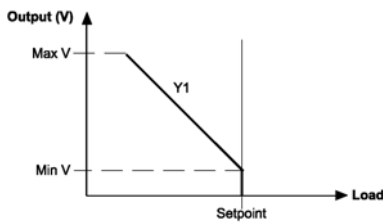
Application No. 3: Single RA 0(2)-10VDC Output
