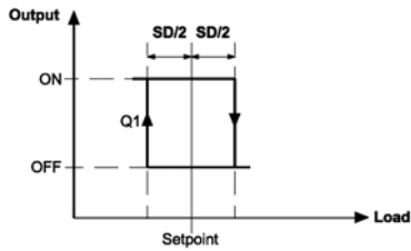
Application No. 1: Single RA On-Off Output
