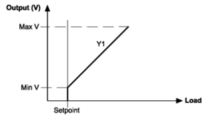
Application No. 4: Single DA 0(2)-10VDC Output
