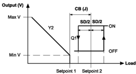
Application No. 7: DA On-Off + RA 0(2)-10 VDC Outputs
