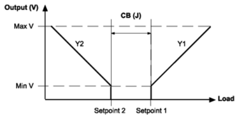
Application No. 5: RA 0(2)-10VDC + DA 0(2)-10 VDC
