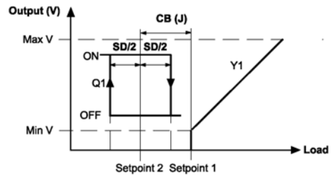
Application No. 6: RA On-Off + DA 0(2)-10 VDC Outputs
