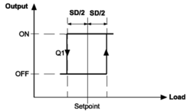
Application No. 2: Single DA On-Off Output
